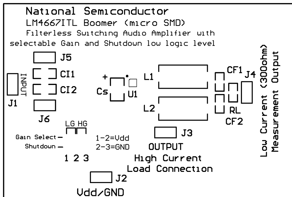
Figure 32. Silk Screen
