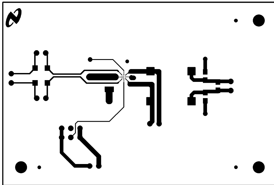
Figure 33. Top Layer
