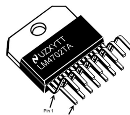
20158302 Plastic Package — 15 Lead TO-220 (for LM4702BTA, LM4702CTA)
