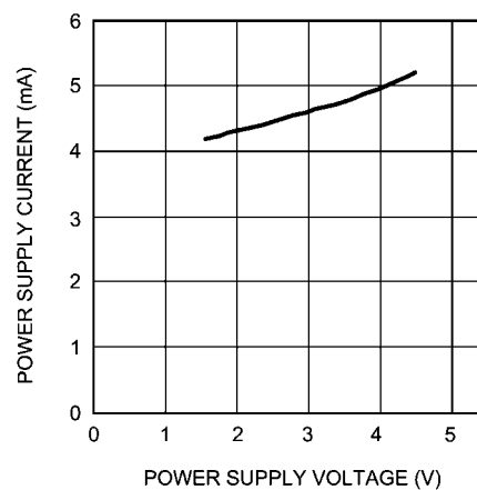
Power Supply Current vs Power Supply Voltage V_{IN} = 0V , Stereo
