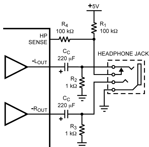
FIGURE 3. Headphone Sensing Circuit
