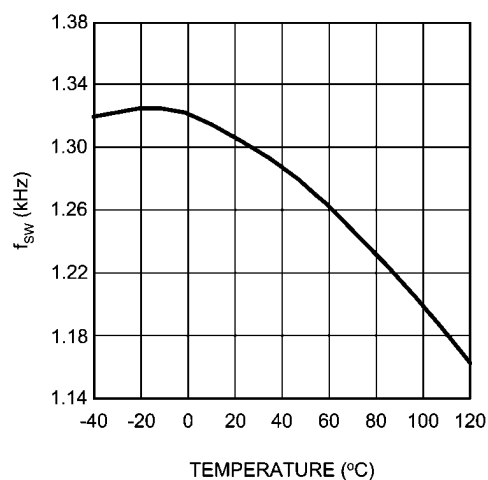
f_{SW} vs. Temperature @ FS = OPEN (-6)
