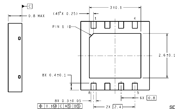
8-Lead LLP Package NS Package Number SDC08A
