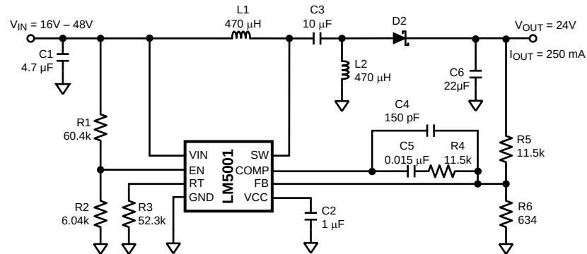
Figure 24. 24V SEPIC
