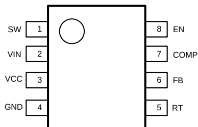
Figure 2. Top View SOIC-8 Package
