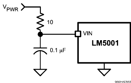
FIGURE 2. Input Transient Protection
