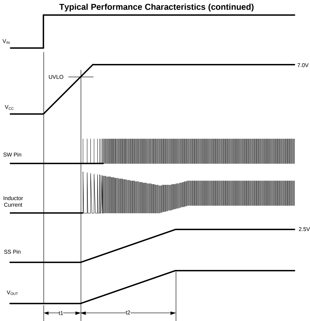
Figure 8. Startup Sequence
