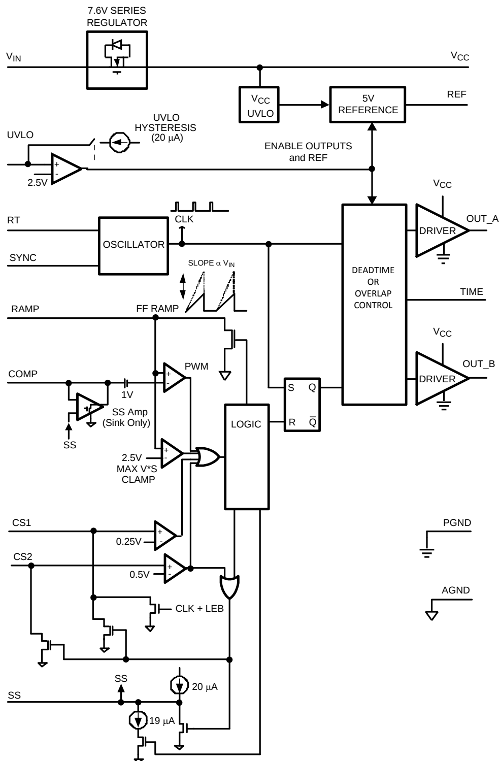
Figure 3. Simplified Block Diagram
