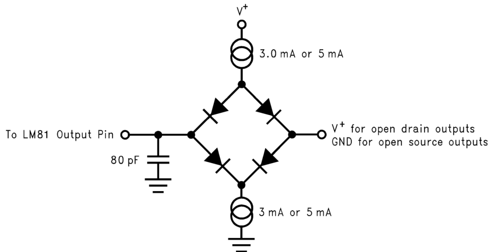
Figure 6. Digital Output Load Test Circuitry
