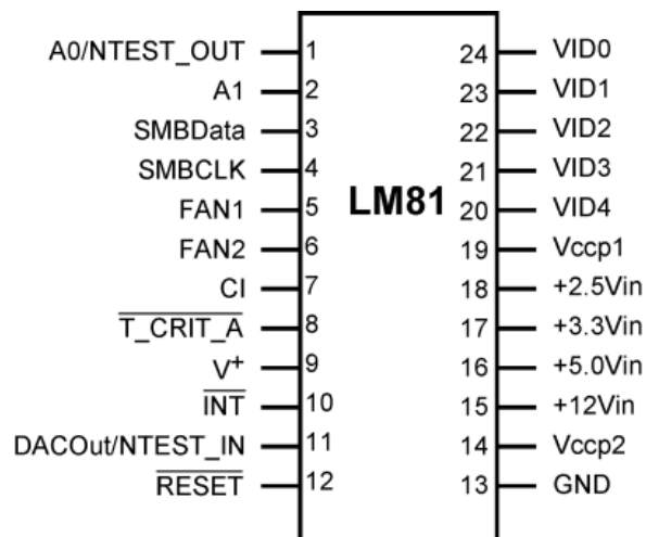
Figure 2. CONNECTION DIAGRAM
