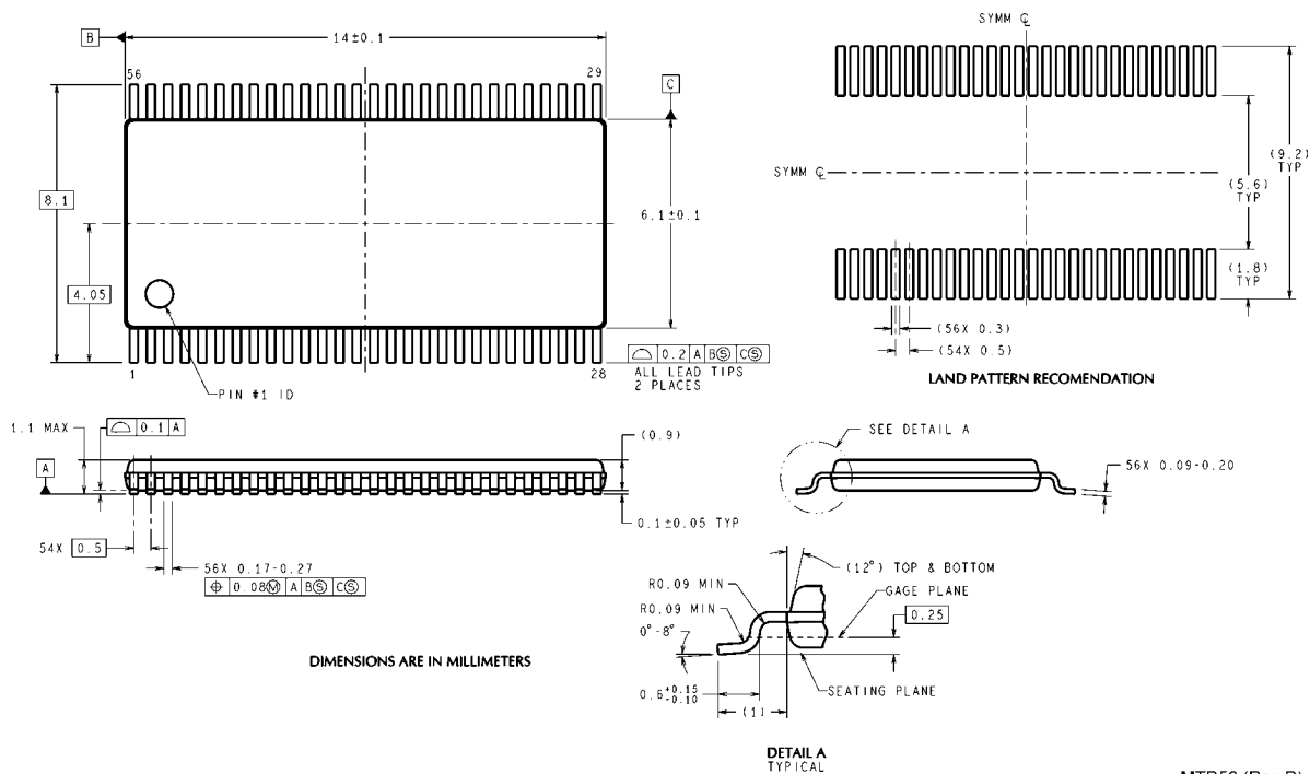
56-Lead Molded TSSOP Package, JEDEC Registration Number MO-153 Variation EE, Order Number LM94C1MT or LM94C1MTX, NS Package Number MTD56
