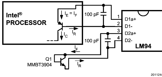
FIGURE 4. Thermal Diode Current Paths
