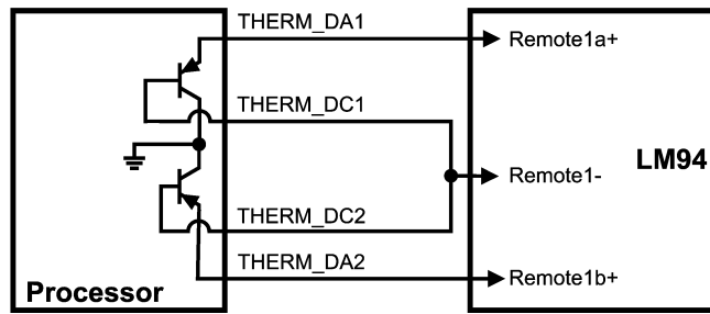
Thermal diode recommended implementation
