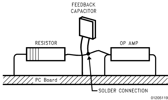
FIGURE 13. Air Wiring
