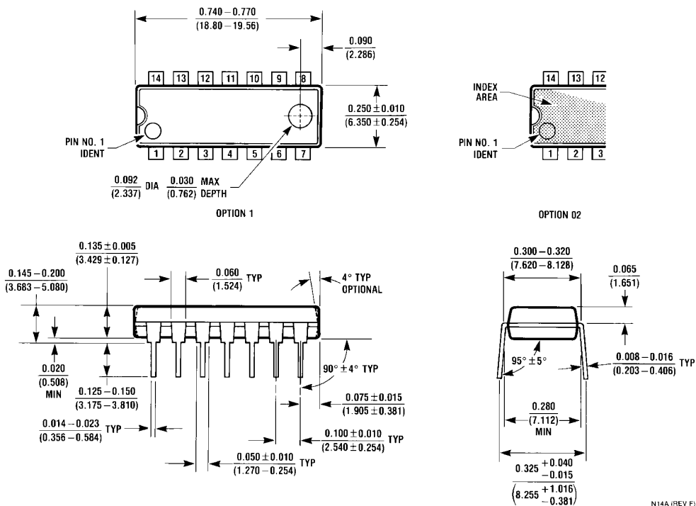
14-Pin Molded Dual-In-Line Pacakge NS Package Number N14A
