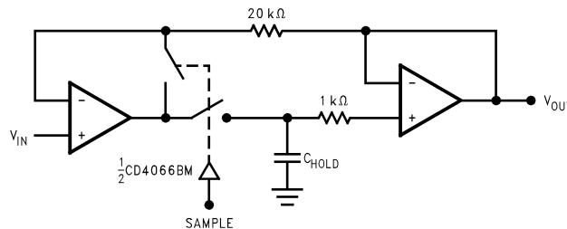
Figure 38. Sample and Hold
