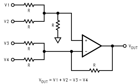
Figure 40. Adder/Subtractor Circuit
