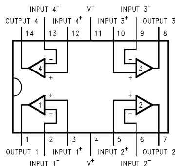
14-Pin DIP/SO
