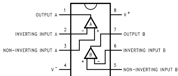
8-Pin DIP/SO/MSOP
