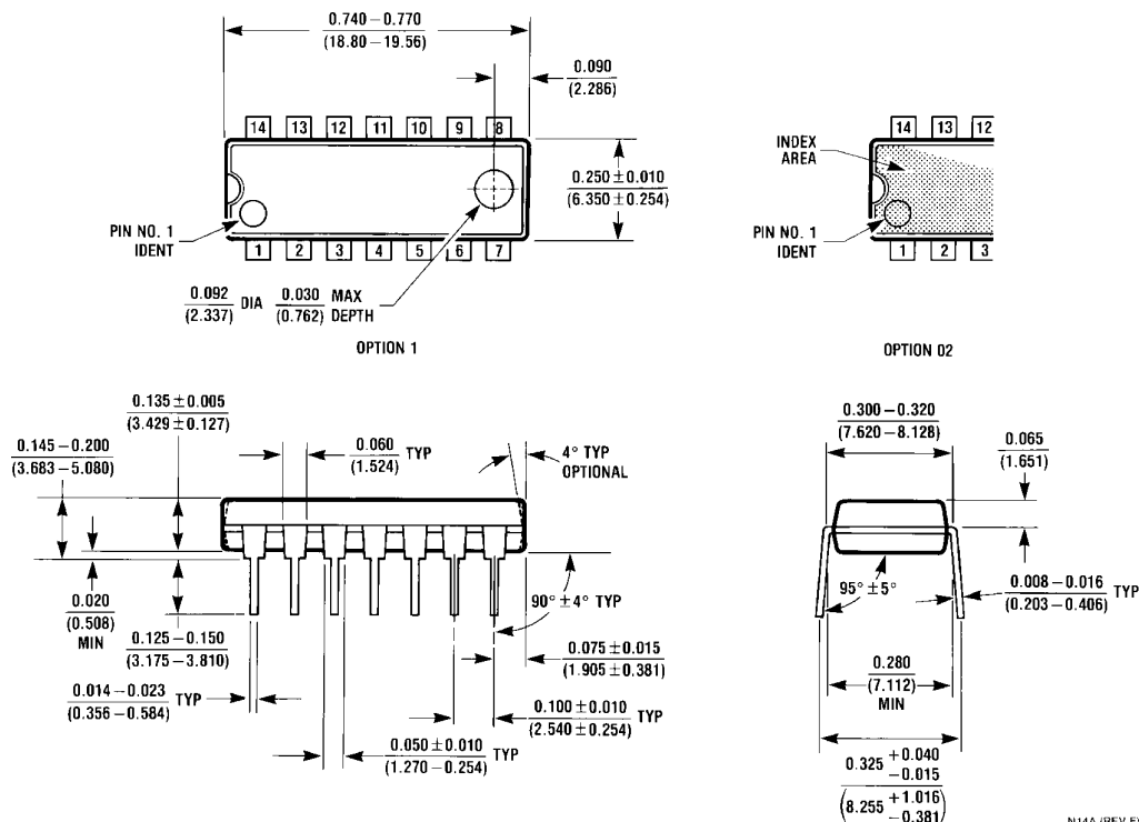
14-Pin Molded Dual-In-Line Package Order Number LMC6574AIN or LMC6574BIN NS Package Number N14A
