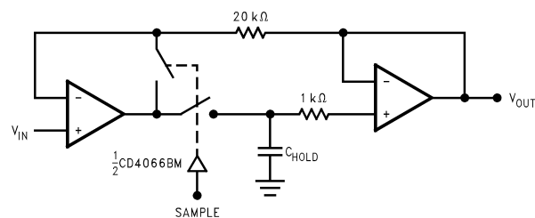
FIGURE 7. Sample and Hold
