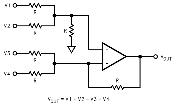
FIGURE 9. Adder/Subtractor Circuit
