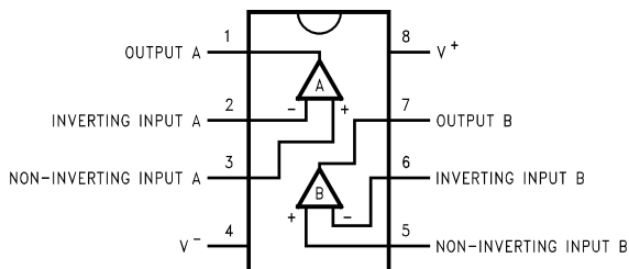
8-Pin DIP/SO/MSOP
