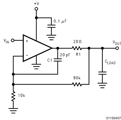
FIGURE 2. LMC6574/2 Noninverting Gain of 10 Amplifier, Compensated to Handle Capacitive Loads
