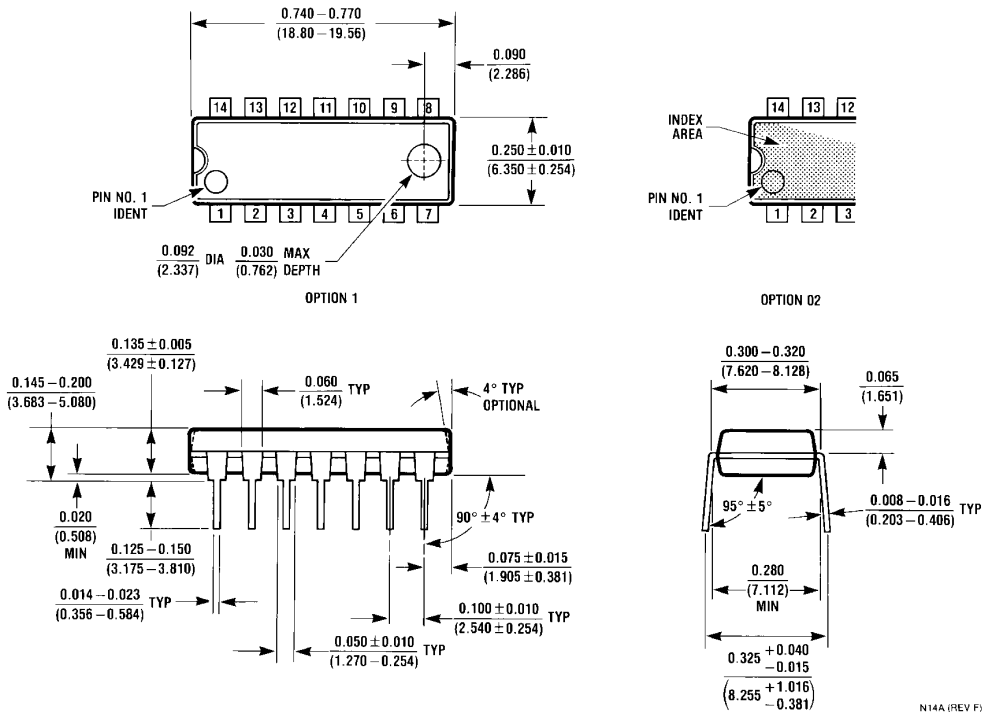
14-Pin MDIP NS Package Number N14A
