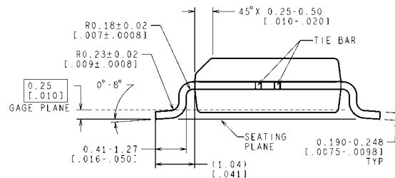
8-Pin SOIC NS Package Number M08A
