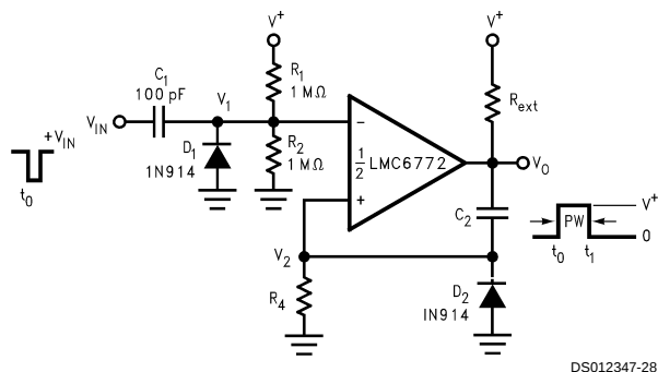
FIGURE 5. One-Shot Multivibrator
