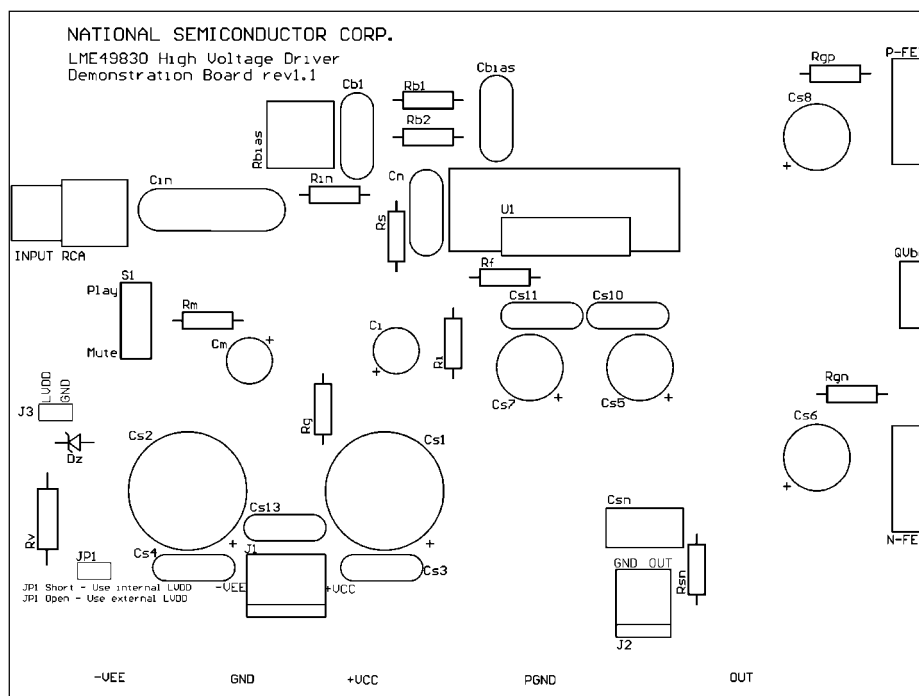
Top Silkscreen
