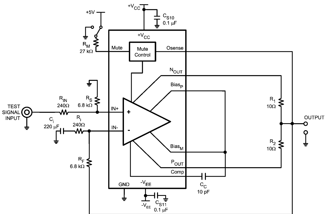
FIGURE 3. LME49830 Test Circuit Diagram
