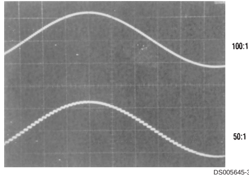
FIGURE 25. The Sampled-Data Output Waveform
