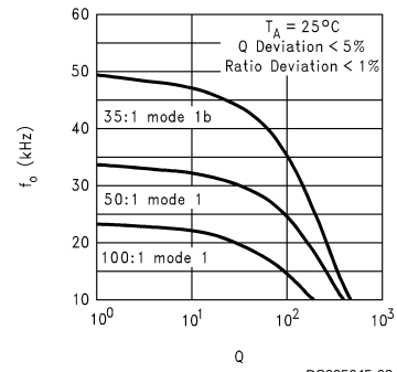
Maximum f_o vs Q at V_s = \pm 2.5V
