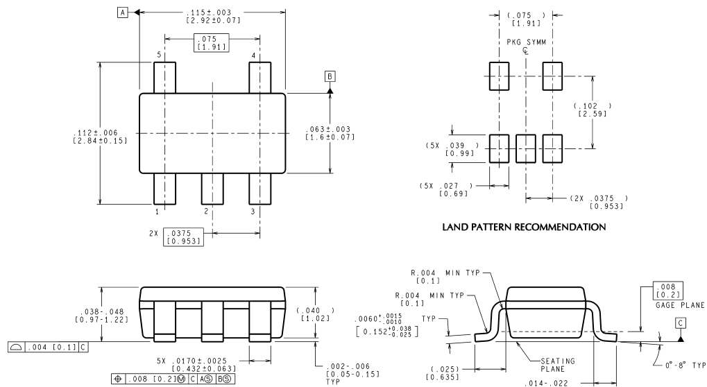
CONTROLLING DIMENSION IS INCH VALUES IN [ ] ARE MILLIMETERS 5-Pin SOT23 NS Package Number MF05A
