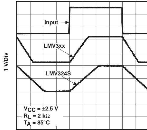
1 \mu\text{s}/\text{Div} Figure 28
