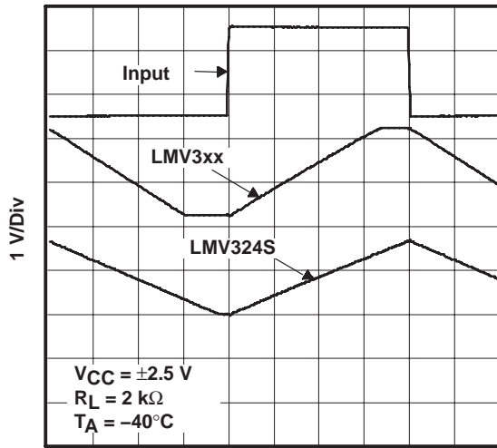
1 \mu\text{s}/\text{Div} Figure 29
