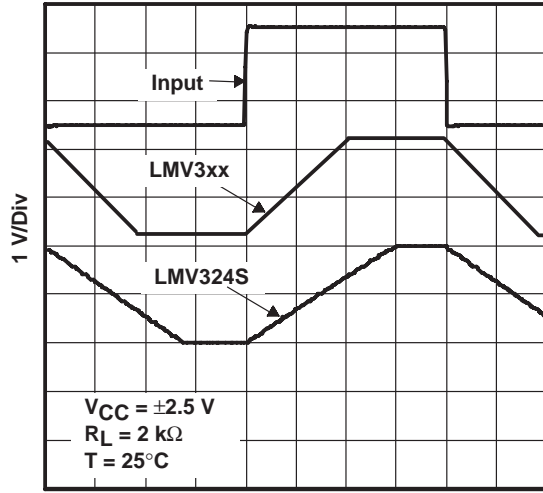
1 \mu\text{s}/\text{Div} Figure 27
