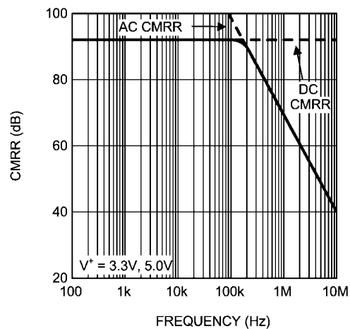
FIGURE 2. CMRR Curve
