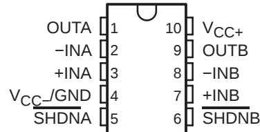
LMV982 . . . DGS (VSSOP/MSOP) PACKAGE
