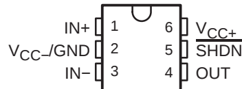
LMV981 . . . RUG (QFN) PACKAGE
