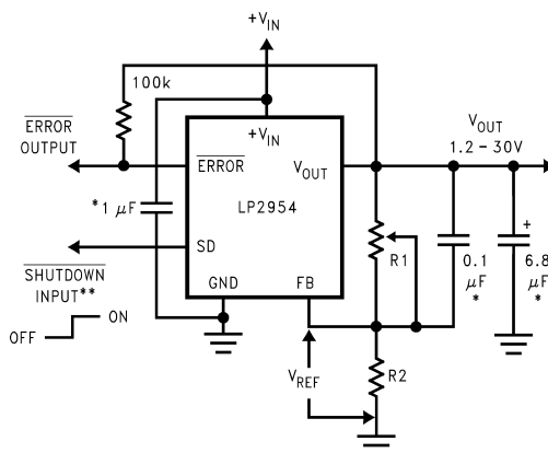
Figure 24. Adjustable Regulator
