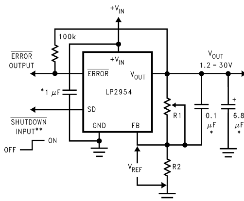
Figure 24. Adjustable Regulator
