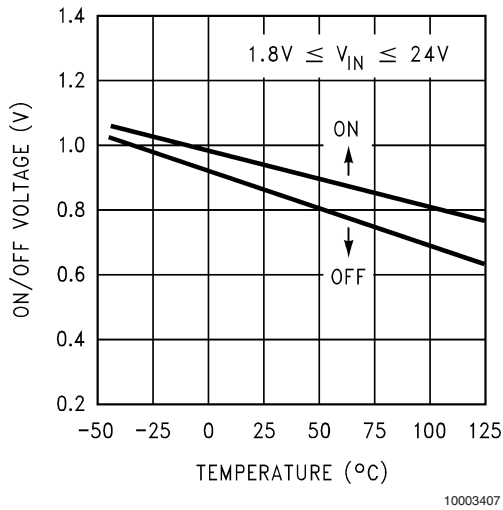
ON/OFF Threshold
