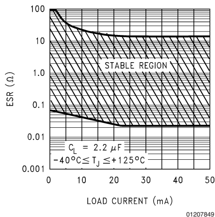
FIGURE 2. 2.2 \mu F ESR Range
