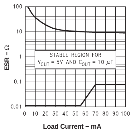
Figure 3. 5-V/10- \mu F ESR Curves
