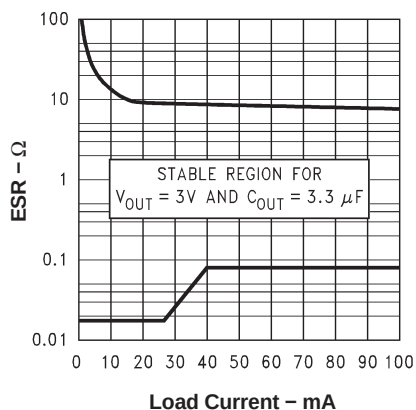
Figure 4. 3-V/3.3- \mu F ESR Curves
