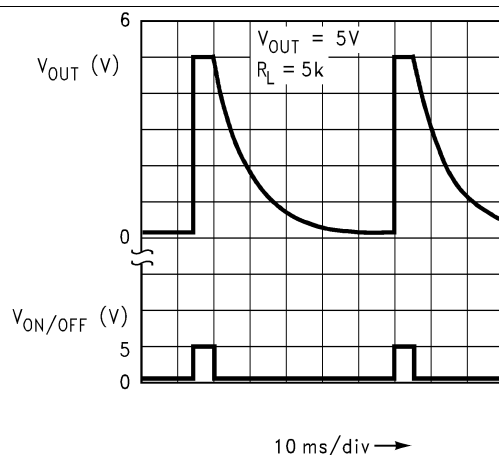
Figure 30. Turnoff Waveform
