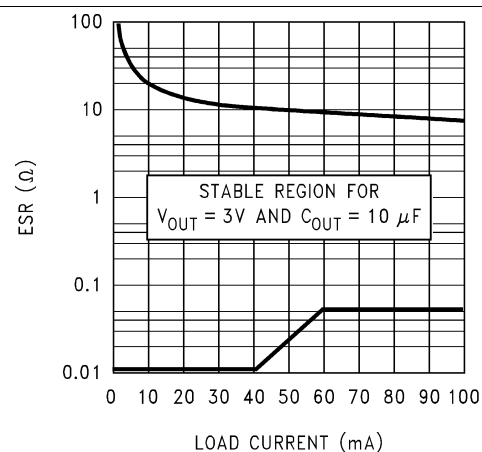
Figure 39. 3-V, 10-μF ESR Curves
