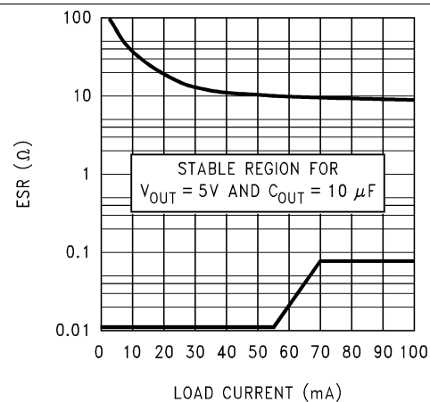
Figure 37. 5-V, 10-μF ESR Curves
