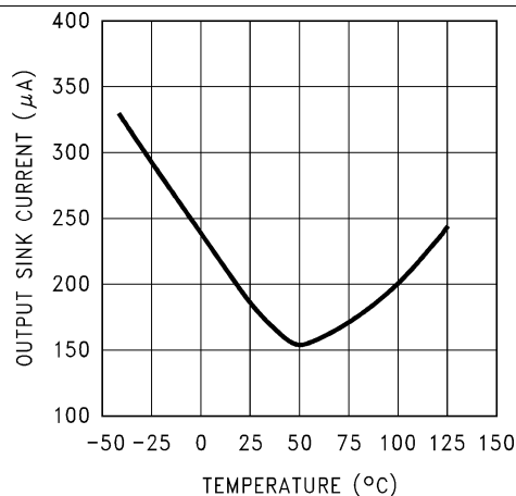
Figure 28. Output Reverse Leakage vs Temperature
