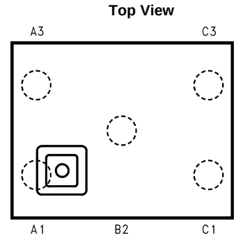
Figure 2. DSBGA Package, 5-Bump Package See Package Numbers YPB0005 and YZR0005
