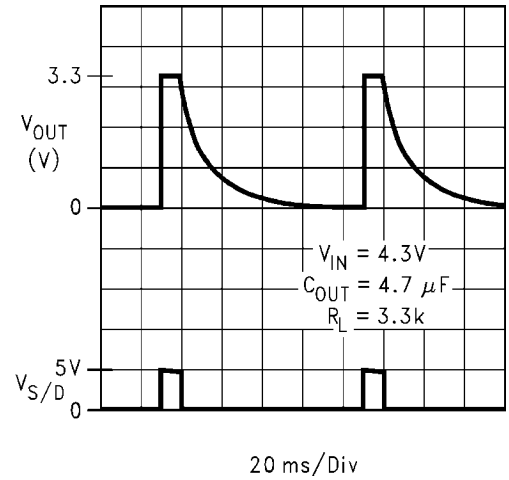
Turn-Off Waveform
