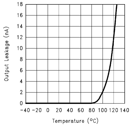
Input to Output Leakage vs Temperature
