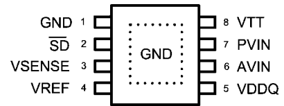
PSOP-8 Layout
