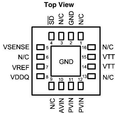
LLP-16 Layout
