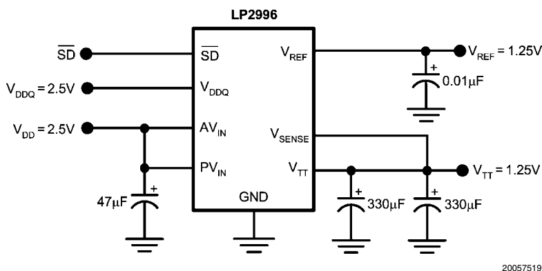
FIGURE 14. Typical SSTL-2 Application Circuit for Motherboards
