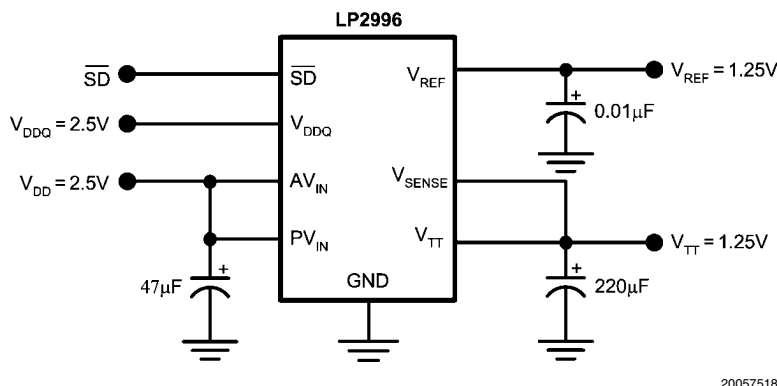
FIGURE 13. Typical SSTL-2 Application Circuit
