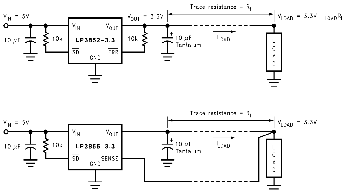
FIGURE 4. Improving remote load regulation using LP3855
