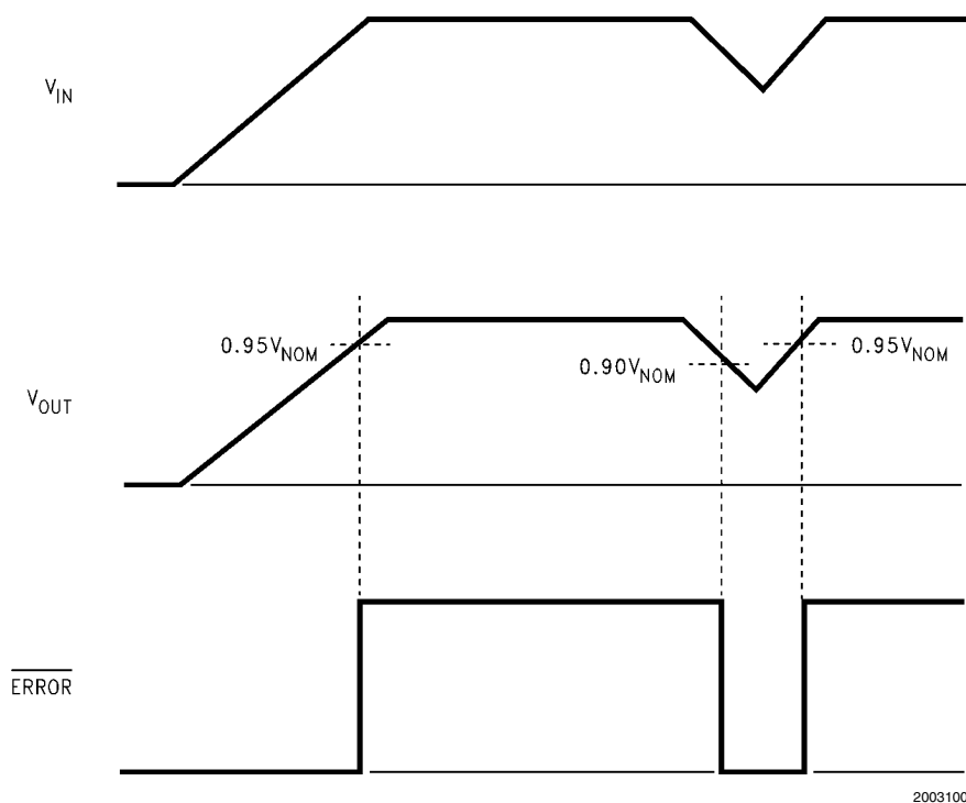
FIGURE 3. \overline{\text{Error}} Flag Operation
