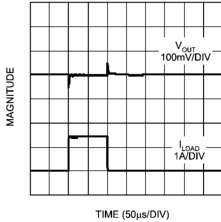
Load Transient Response C_{IN} = C_{OUT} = 100\mu F , TANTALUM
