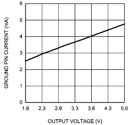
Ground Current vs Output Voltage I_L = 1.5\text{A}
