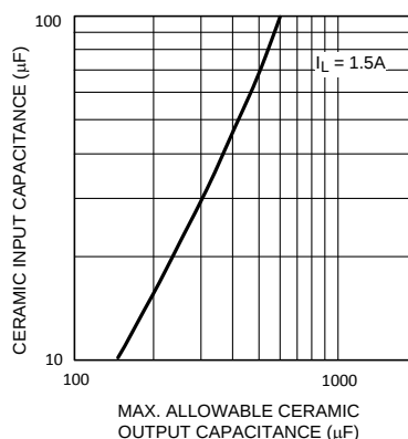
Figure 22. Maximum Ceramic Output Capacitance vs Ceramic Input Capacitance
