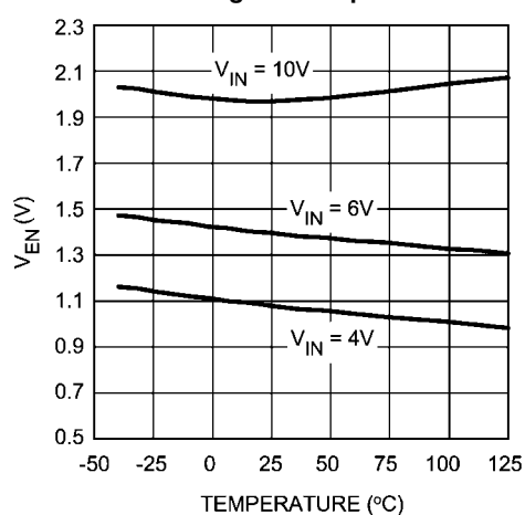
Enable Voltage vs Temperature
