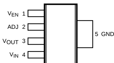
Figure 1. SOT-223 (LP38693MP-ADJ) – Top View See Package Number NDC0005A
