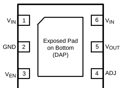
Figure 3. 6-Lead WSON (LP38693SD-ADJ) – Top View See Package Number NGG0006A
