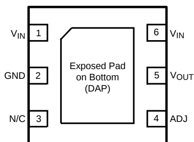
Figure 2. 6-Lead WSON (LP38691SD-ADJ) – Top View See Package Number NGG0006A
