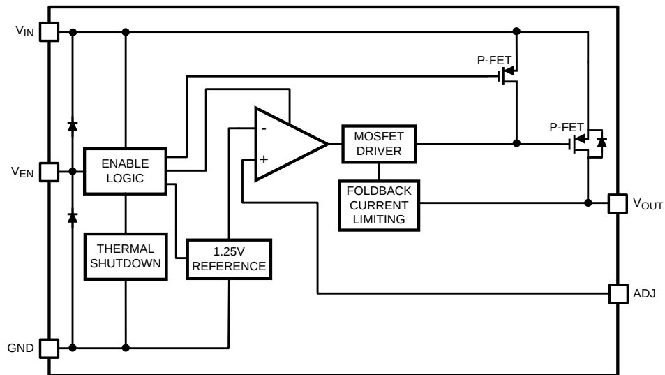
Figure 5. LP38693-ADJ Functional Diagram (SOT-223, WSON)
