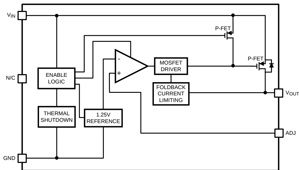
Figure 4. LP38691-ADJ Functional Diagram (WSON)
