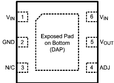
6-Lead LLP, Top View LP38690SD-ADJ
