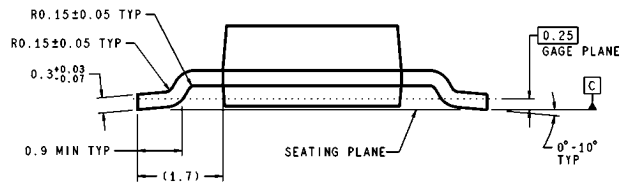
SOT-223 Package NS Package Number MP05A
