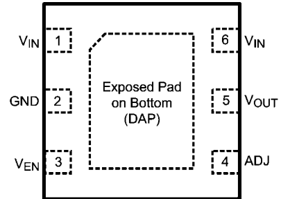
6-Lead LLP, Top View LP38692SD-ADJ
