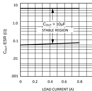
Figure 18. ESR Curve
