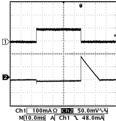
Load Transient (LDO1) 3.6 Vin, 3.3 Vout, 0 – 100 mA load
