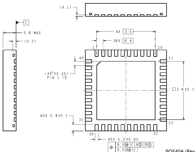
40-Pin Leadless Leadframe Package NS Package Number SQF40A
