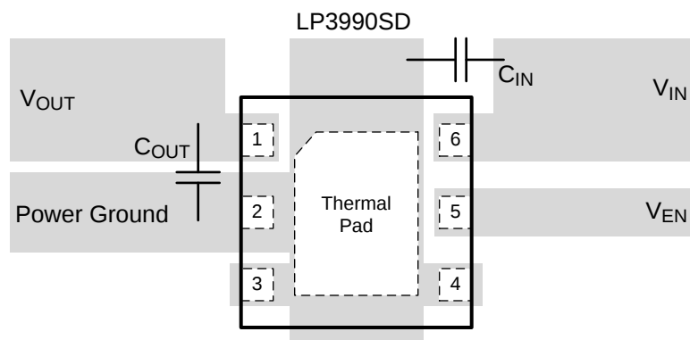
Figure 19. LP3990 WSON Layout
