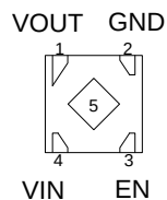
4-pin X2SON Package (Bottom View)
