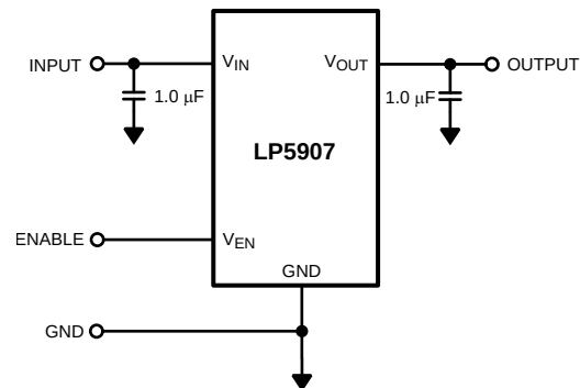
Typical Application Circuit
