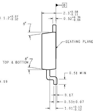
3-Pin DPAK NS Package Number TD03B
