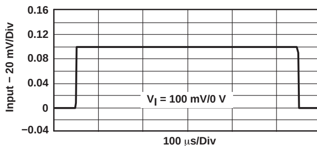
NONINVERTING SMALL-SIGNAL PULSE RESPONSE
