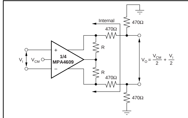
FIGURE 10. Grounded Load Attenuation.
