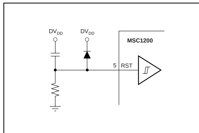
FIGURE 10. Typical Reset Circuit.
